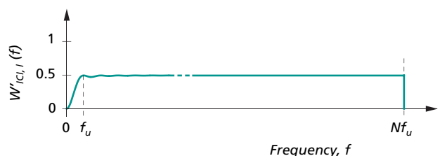
Figure 9 The simplified one-sided weighting function for ICI into an edge carrier.
