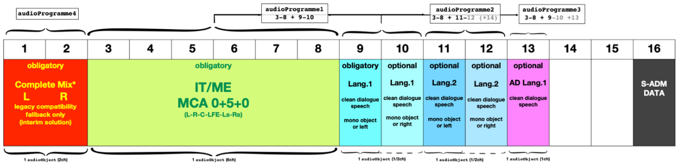
Figure C1: Tracks allocation according to Template 1
