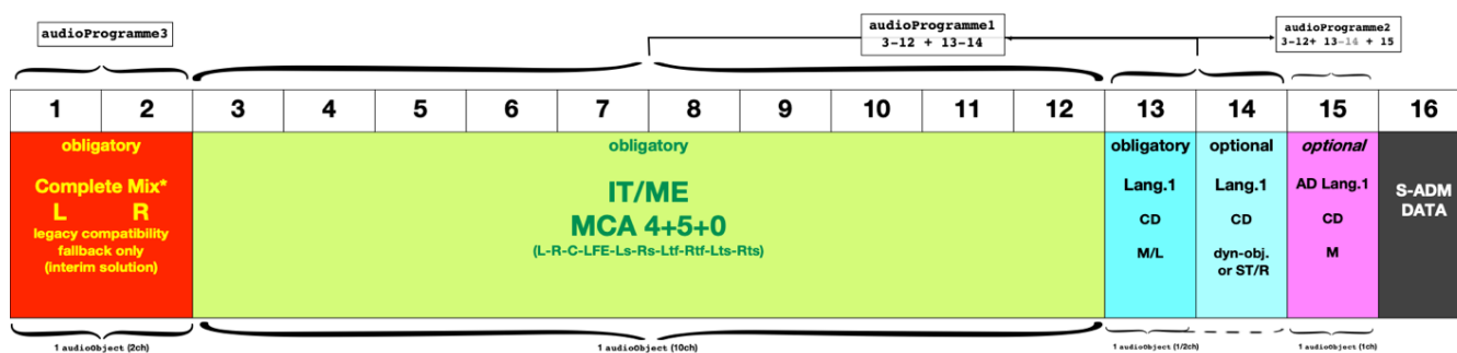
Figure C3: Tracks allocation according to Template 2
