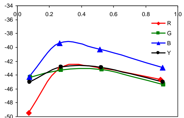
Figure 5 Noise at 0dB, ununsuppressed
