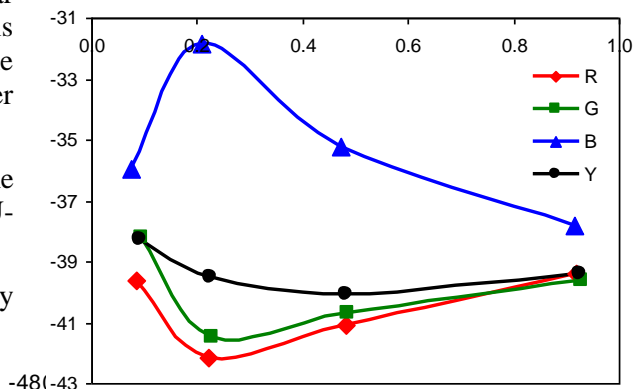
Figure 7 Noise at +12dB gain, suppression on
