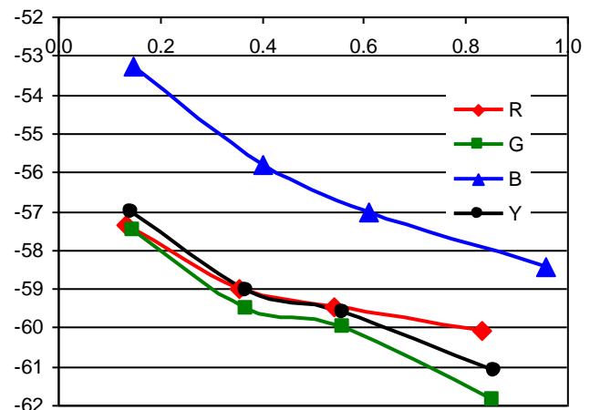
Figure 4 Camera noise
