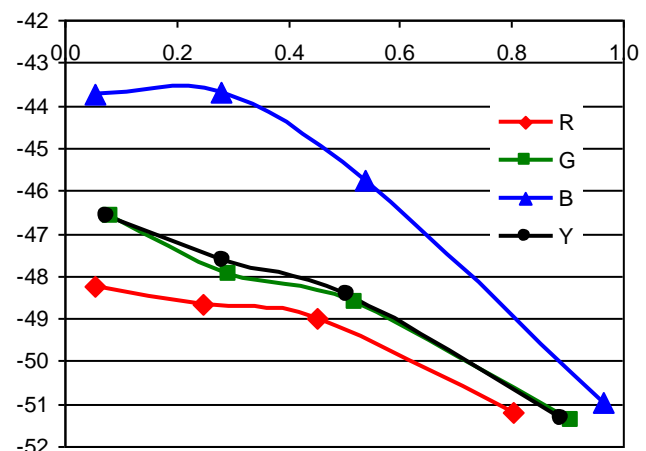
Fig. 4 Camera noise
