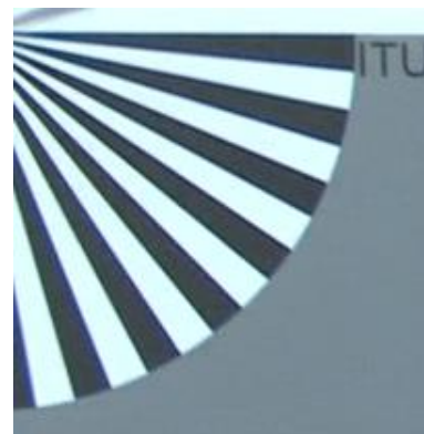
Figure 6 Corner aberration
