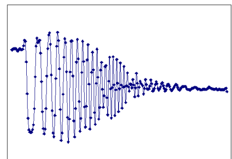
Figure 8, horizontal waveform
