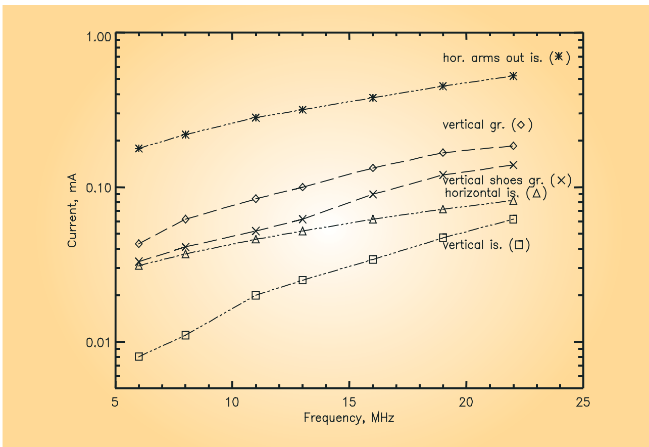
Figure 5.7 Calculated wrist current values. These are for vertically and horizontally polarized fields in the standard and arms horizontally out to the side posture under isolated, shod and grounded conditions. The incident electric field is 1 V m -1 (rms).
