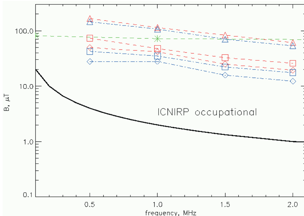
Figure 6.3 Comparison of ICNIRP occupational exposure magnetic flux density reference levels (solid line) with calculated fields required to generate basic restrictions. The green asterisks are for current density. The blue symbols are for leg SAR, the red symbols are for whole-body SAR. Diamonds are for grounded conditions, squares are with shoes and triangles for isolated conditions.
