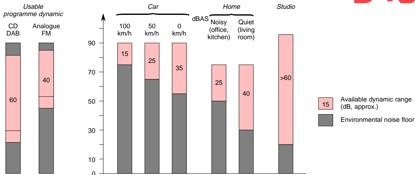
Figure 2 Reproduced dynamic range.
