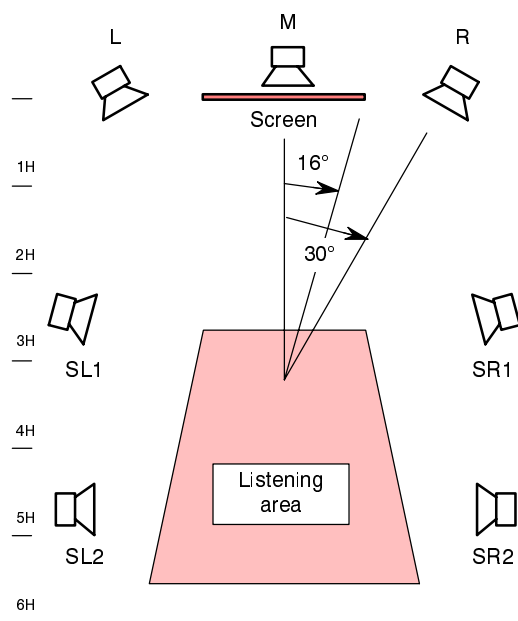
Figure 4 Loudspeaker arrangement for sound reproduction
